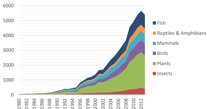
N publications / year
