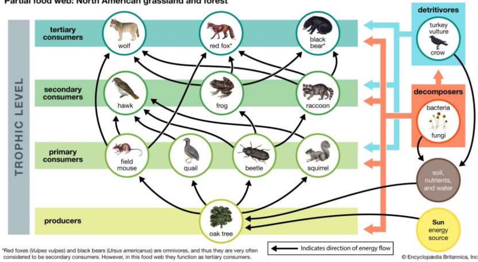
Partial food web: North American grassland and forest
